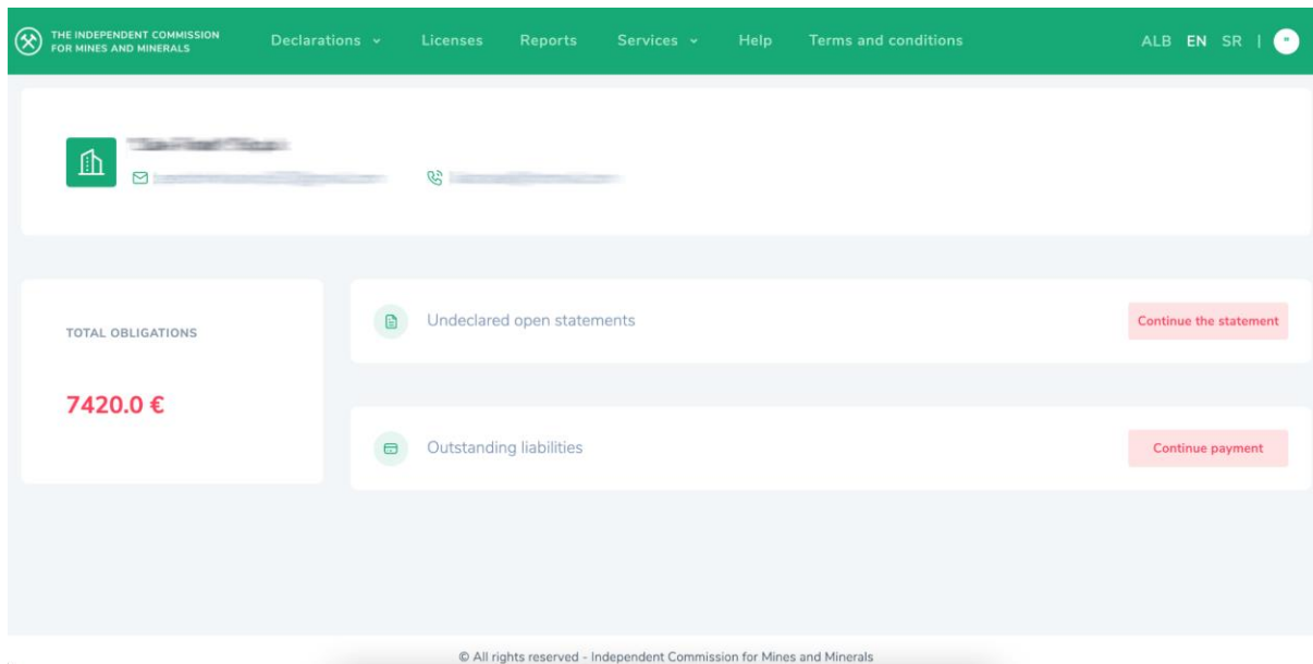
Figure 3: Entity overview
